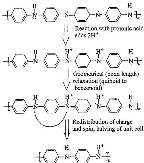
Fig. 4 Protonation induced spin unpairing in polyaniline; conversion from insulator to metal with no change in the number of electrons The counterion is not shown.
