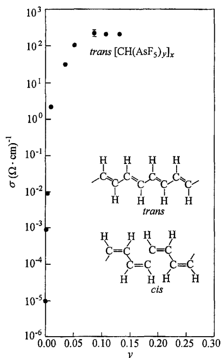
Fig. 2 Electrical conductivity of trans -(CH) x as a function of (AsF 5 ) dopant concentration The trans and cis polymer structures are shown.
