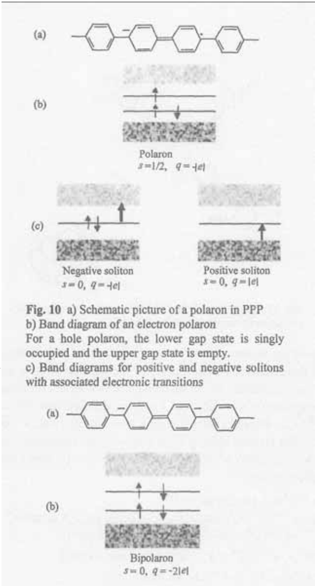
Fig. 11 Bipolarons in polymer with non-degenerate ground state a) Schematic picture of a negative bipolaron in PPP b) Band diagram for a negative bipolaron For a positive bipolaron, both gap states are unoccupied.
