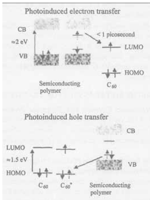
Fig. 13 Energy band diagram for photoinduced electron transfer and photoinduced hole transfer between semiconducting polymers and C_{60}
