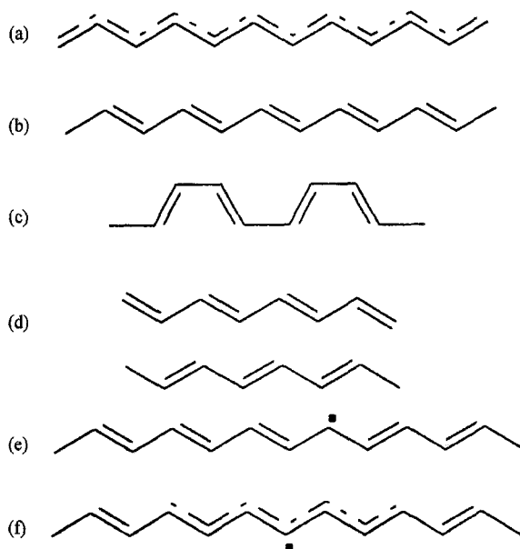
Fig. 6 Polyacetylene: a) undimerized structure, b) dimerized structure due to the Peierls instability, c) cis -polyacetylene, d) degenerate A and B phases in trans -polyacetylene, e) soliton in trans -polyacetylene; the soliton structure is actually delocalized over approx 10–14 carbon-carbon bonds, as shown in f)
