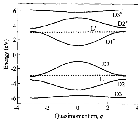
Fig. 9 Electronic band structure of PPV
