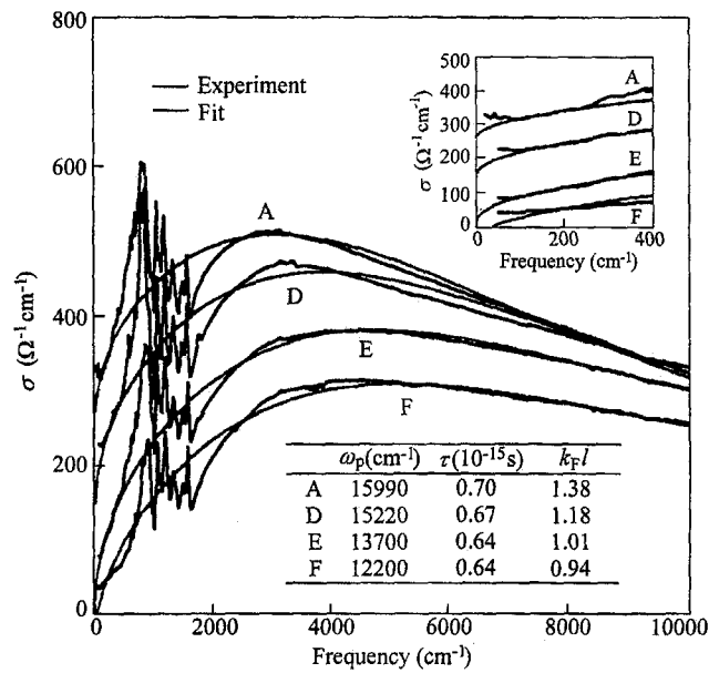
Fig. 14 Frequency dependent conductivity, \sigma(\omega) , for PPy-PF 6 . The inset shows the far-IR data in greater detail.
