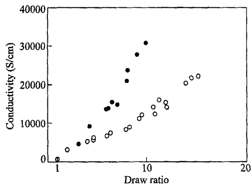
Fig. 15 Electrical conductivity of iodine-doped polyacetylene (parallel to the draw axis) versus draw ratio; solid points, thin films of thickness 3–5 \mu\text{m} ; open circles, films of thickness 25–30 \mu\text{m}
