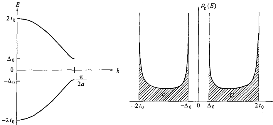
Fig. 7 Electronic structure of semiconducting polyacetylene
