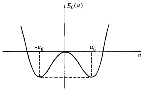
Fig. 8 Total energy of the dimerized polyacetylene chain; note the double minimum associated with the spontaneous symmetry breaking and the two-fold degenerate ground state
