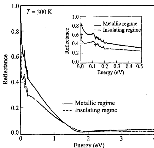
Fig. 5 Reflectance spectra of PPy-PF 6 near the metal-insulator transition. Inset shows the low energy spectra with expanded scale.
